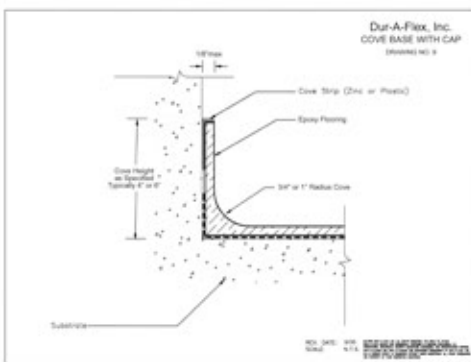
cove base w cap06.pdf
