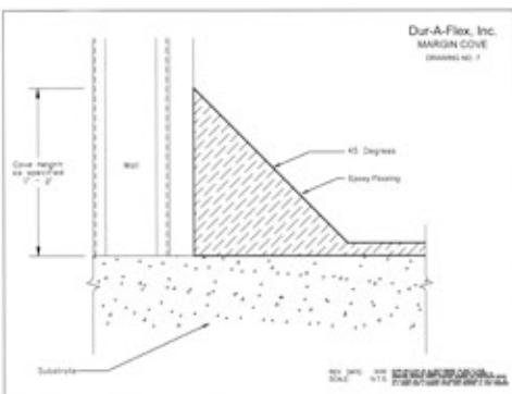
margin cove06.pdf
