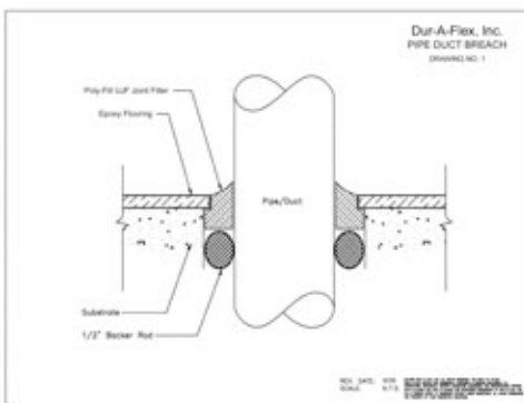
pipe duct breach06.pdf
