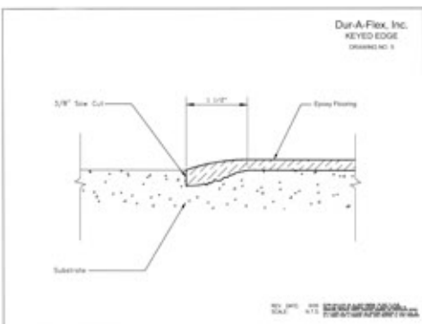
keyed edge06.pdf
