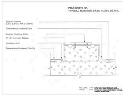
PCrete HF base plate detail.pdf
