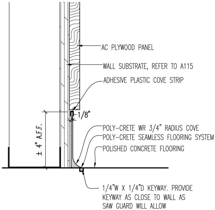
9D A125 POLYCRETE BASE DETAIL @ PLYWOOD 3" = 1'-0"
